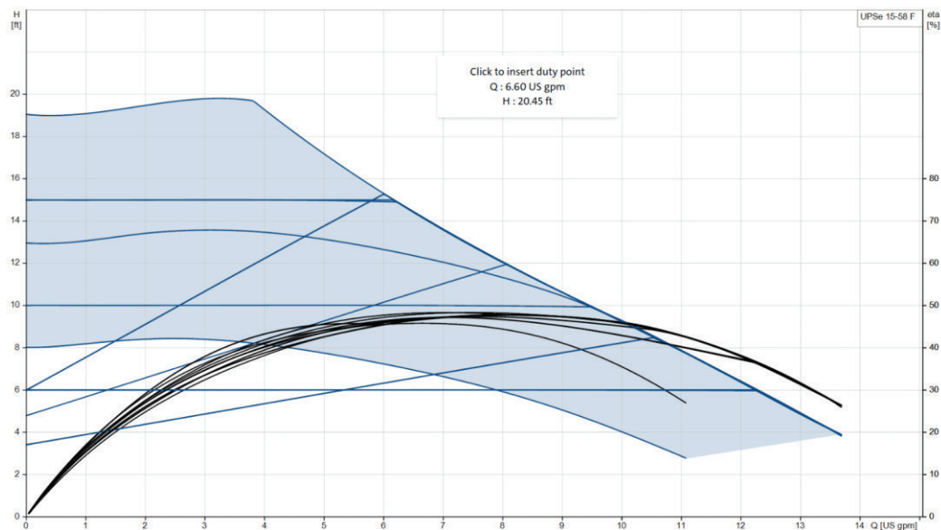
GEP15-58 – Proportional Control Pump Curve
