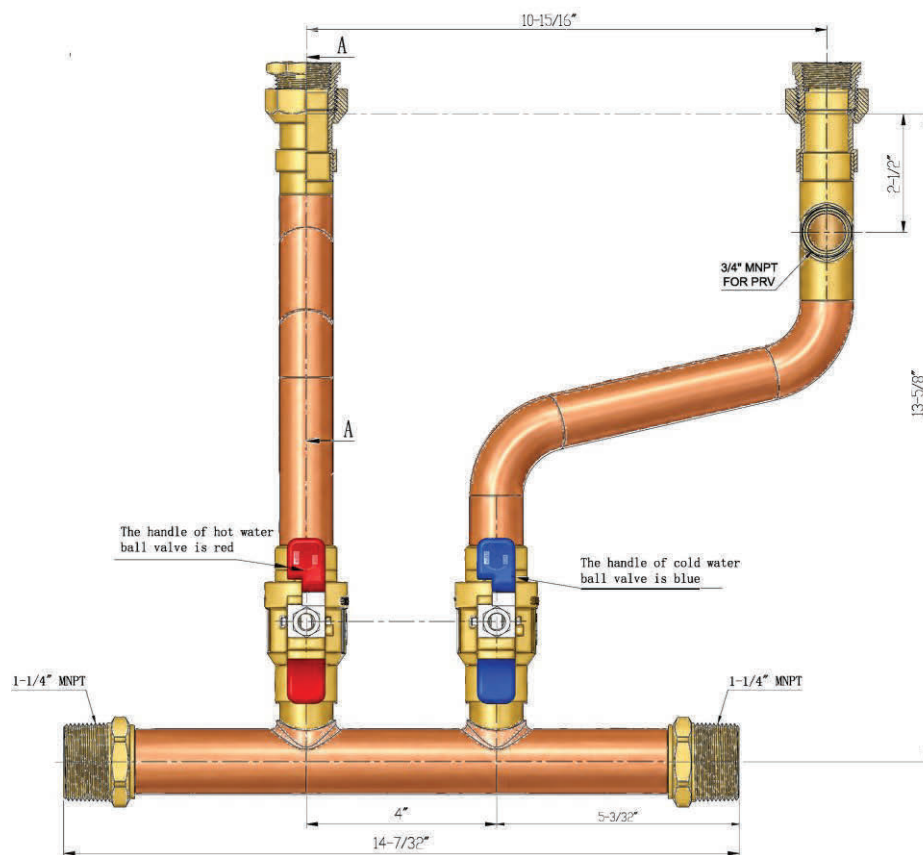
PSM 114 – Primary Secondary Manifold Specifications:
